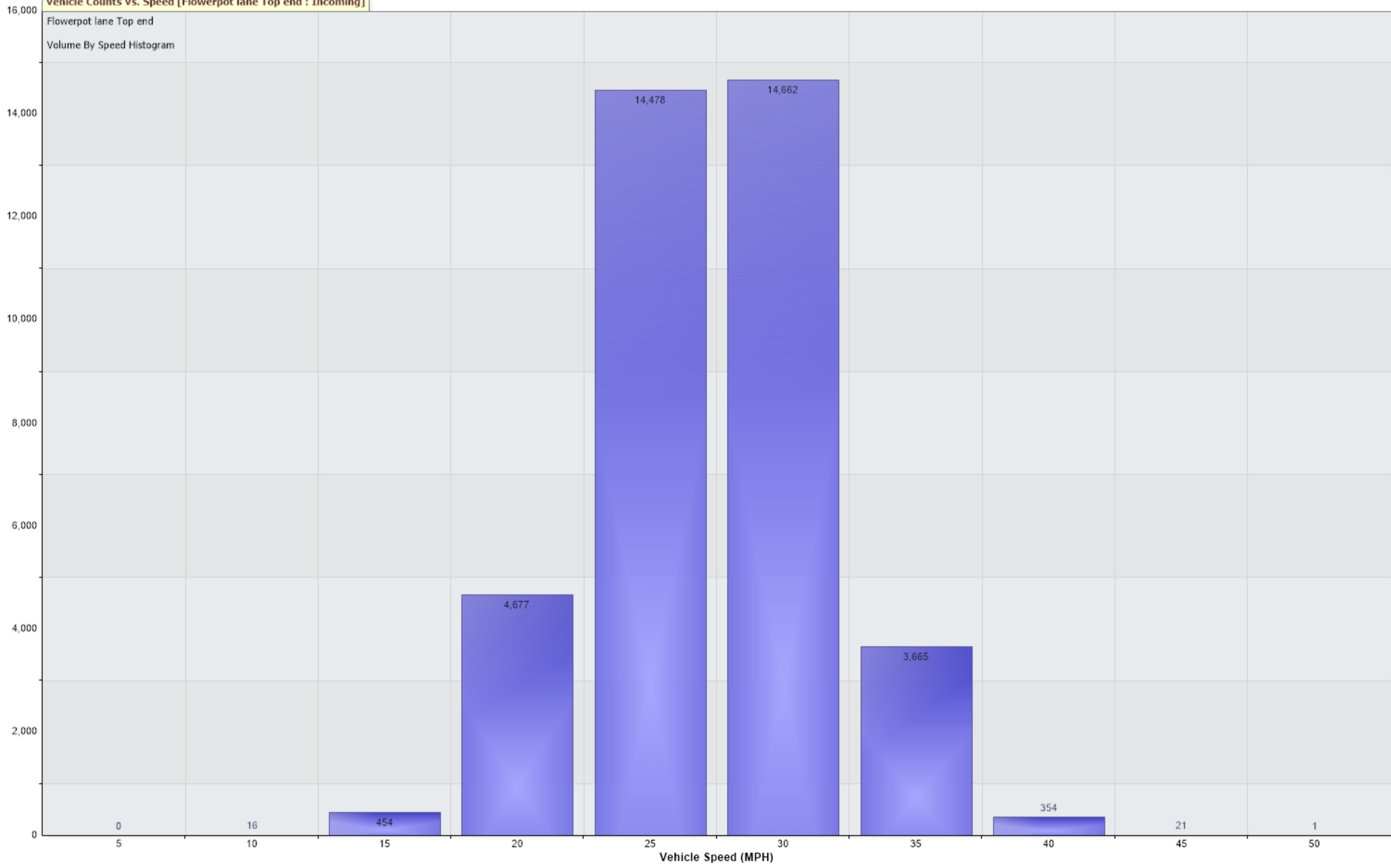
Vehicle Counts Vs. Speed [Flowerpot lane Top end : Incoming]
